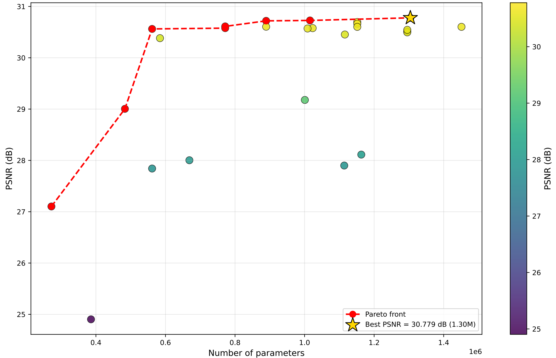
PSNR vs #Parameters — OmniSR
